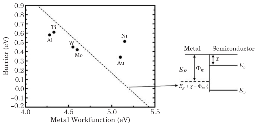
Figure 3.3 Measured Schottky barrier heights for traditional contacts between silicon and various metals. The dashed line represents the behavior predicted from Eq. (3.1), which corresponds to the direct band alignment between the metal Fermi level and the semiconductor valence and conduction bands, as shown in the schematic on the right. This simple model fails to explain the experimental data. See text for details.
