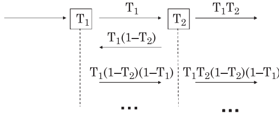
Figure 4.47 Illustration of the procedure to calculate the total transmission probability across two scatterers in series.
