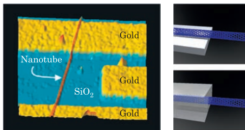
Figure 3.2 Left: atomic force microscope image of a carbon nanotube forming “side contacts” to gold electrodes. Figure from Ref. [3]. Right: sketch of two possible realizations of side contacts: the top figure shows a nanotube laying on a metal contact and the bottom figure shows a nanotube embedded in the metal.
