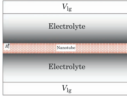
Figure 8.15 Cross-section of the system for calculation of the capacitance of a liquid gate. A carbon nanotube is immersed in an electrolyte, and a reference potential V_{lg} is set far from the nanotube. The gray shading represents the distribution of charge in the electrolyte that screens the charge on the nanotube.
