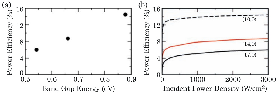
Figure 7.20 (a) shows the maximum power efficiency at 3000 W/cm 2 as a function of nanotube bandgap, and (b) shows the maximum efficiency versus optical power density. Figure from Ref. [14].
