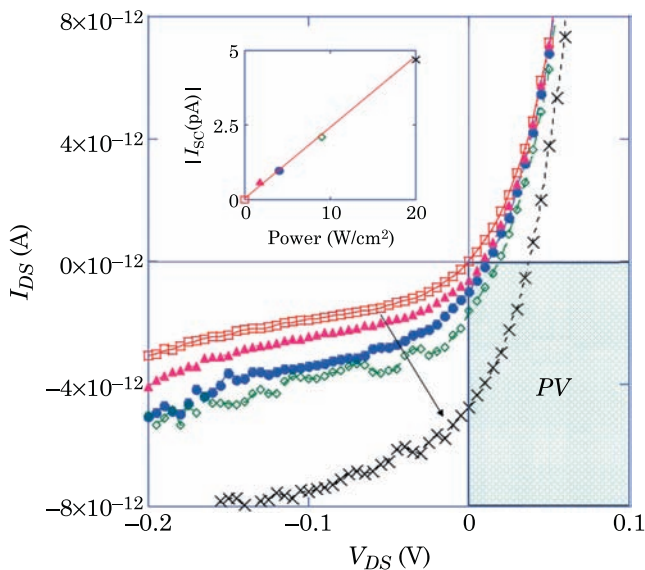
Figure 7.24 Photovoltaic properties of a carbon nanotube p - n junction. The main panel shows the progression of the current–voltage characteristics under increasing light intensities. The inset shows the dependence of the short-circuit current on the light intensity. Figure from Ref. [18].
