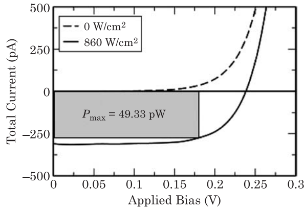
Figure 7.18 Current–voltage characteristics for a (17,0) nanotube p – n junction under illumination, for a photon energy of 0.56 eV. Dashed line is for the dark junction. The optical power density is 860 W/cm 2 . The maximum power generated by the illuminated device is P_{\max} = 49.33 pW as shown by the shaded area. Figure from Ref. [14].
