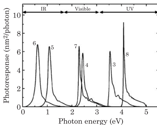
Figure 7.15 Calculated photoresponse of a nanotube p - n junction. Each of the peaks corresponds to a different band of the nanotube, labeled with the value of the angular momentum. Figure from Ref. [13].
