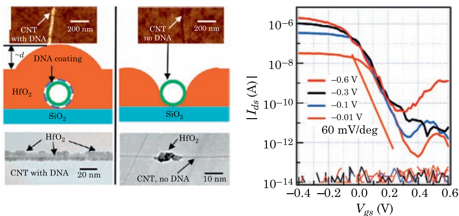
Figure 4.23 Left image: growth of \text{HfO}_2 by atomic layer deposition on carbon nanotubes with and without a DNA coating. Top images in both panels are atomic force microscope images of carbon nanotubes with about 5 nm of \text{HfO}_2 . Middle panels are sketches of the expected wetting behavior. The bottom panels show transmission electron microscopy images of a 5 nm layer of \text{HfO}_2 on the carbon nanotubes. Good wetting is seen in the case of DNA-functionalized nanotubes. Right image: transfer characteristics of a carbon nanotube transistor with 3 nm of \text{HfO}_2 as the gate dielectric. The subthreshold swing approaches the theoretical room-temperature limit of 60 mV/decade. Figures from Ref. [19].
