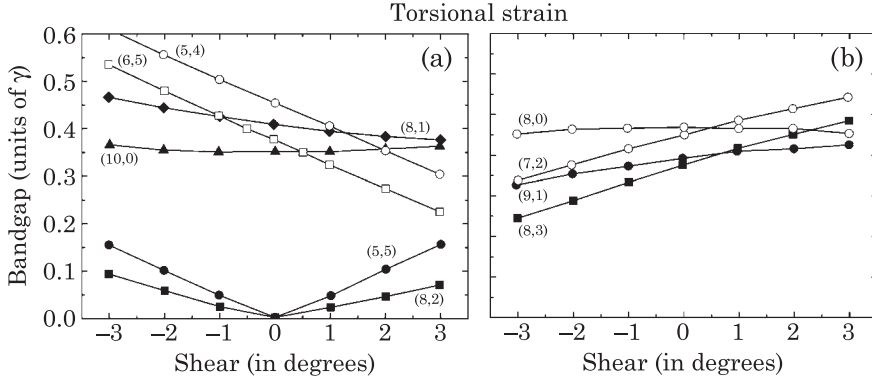
Figure 5.9 Bandgap change with torsional strain. (a) Armchair nanotubes have the largest change in bandgap under torsional strain, and zigzag tubes are the least affected. dE_g/d\sigma is negative for nanotubes satisfying n - m = 3I + 1 . (b) dE_g/d\sigma is positive for nanotubes satisfying n - m = 3I - 1 . All calculations are within the single \pi orbital approximation. Figure after Ref. [9].
