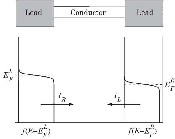
Figure 2.3 Sketch of a ballistic conductor between two leads as well as the finite-temperature Fermi distributions in each lead. The current through the conductor can be considered as the sum of right and left currents.
