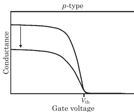
Figure 8.7 Illustration of the impact of increased scattering on the transfer characteristics of a p -type carbon nanotube field-effect transistors. The threshold voltage is unchanged, but the conductance in the ON state and the subthreshold swing decrease.
