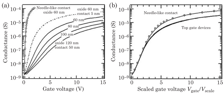
Figure 4.21 (a) Influence of transistor geometry on the device characteristics of Schottky barrier nanotube transistors. The four right-most curves correspond to different thicknesses of the oxide above the nanotube, as labeled, with all other parameters as in Fig. 4.18. (The curve for 100 nm is the same as that in Fig. 4.18 (b) for a Schottky barrier height of 0.3 eV.) The dot-dashed curve shows the conductance when the contact thickness is reduced to 5 nm. The curve at the left corresponds to a needle-like metal electrode and cylindrical gate. Open circles are calculated as for the other curves, solid curve uses the exact electrostatic kernel. All calculations are at room temperature. (b) The graph shows the same curves, but for each curve the gate voltage is rescaled by the voltage at which the conductance is 10^{-8} S. (The five rightmost curves cannot be distinguished on this scale, forming a single line). Figure from S. Heinze.
