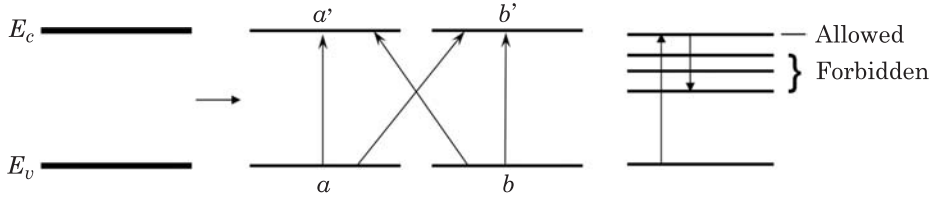
Figure 7.7 Left: illustration of the doubly degenerate conduction and valence bands in a single-wall carbon nanotube. Middle: the four possible optical transitions from a single-particle picture. Right: in the presence of the electron-hole interaction, the four degenerate single-particle transitions are split. The highest energy state is optically allowed, while the lowest three are not. Excitation of an electron to the highest energy state is followed by relaxation into the lower energy states, which prevents photoluminescence. Figure from Ref. [7].
