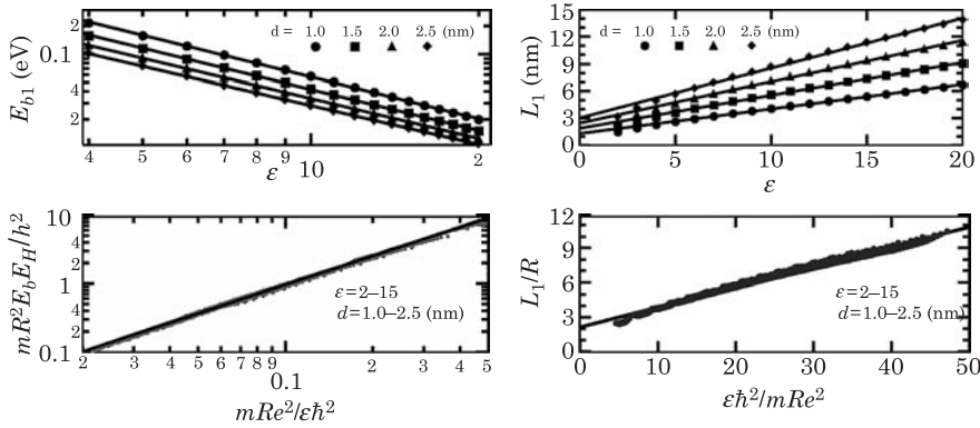
Figure 7.8 Scaling relationships for excitons in semiconducting carbon nanotubes. The left panels show the dependence of the exciton binding energy E_{b1} on the dielectric constant of the surrounding medium \epsilon , and the scaling with nanotube radius R and effective mass m . Figures from V. Perebeinos.
