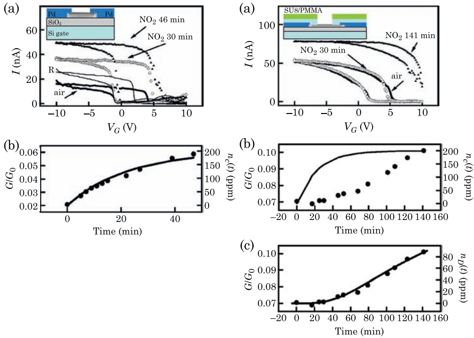
Figure 8.10 Transfer characteristics of a carbon nanotube field-effect transistor upon exposure to \text{NO}_2 . The left and right panels show the results without and with a SU-8/PMMA protective layer on the contacts. The panels labeled (b) in both figures compare the measured time-dependence of the conductance with the expected time dependence of the concentration inside the chamber (solid line). The bottom right panel shows a comparison of the measured conductance with the calculated concentration of \text{NO}_2 from diffusion across the SU-8/PMMA layer. Figures from Ref. [14].
